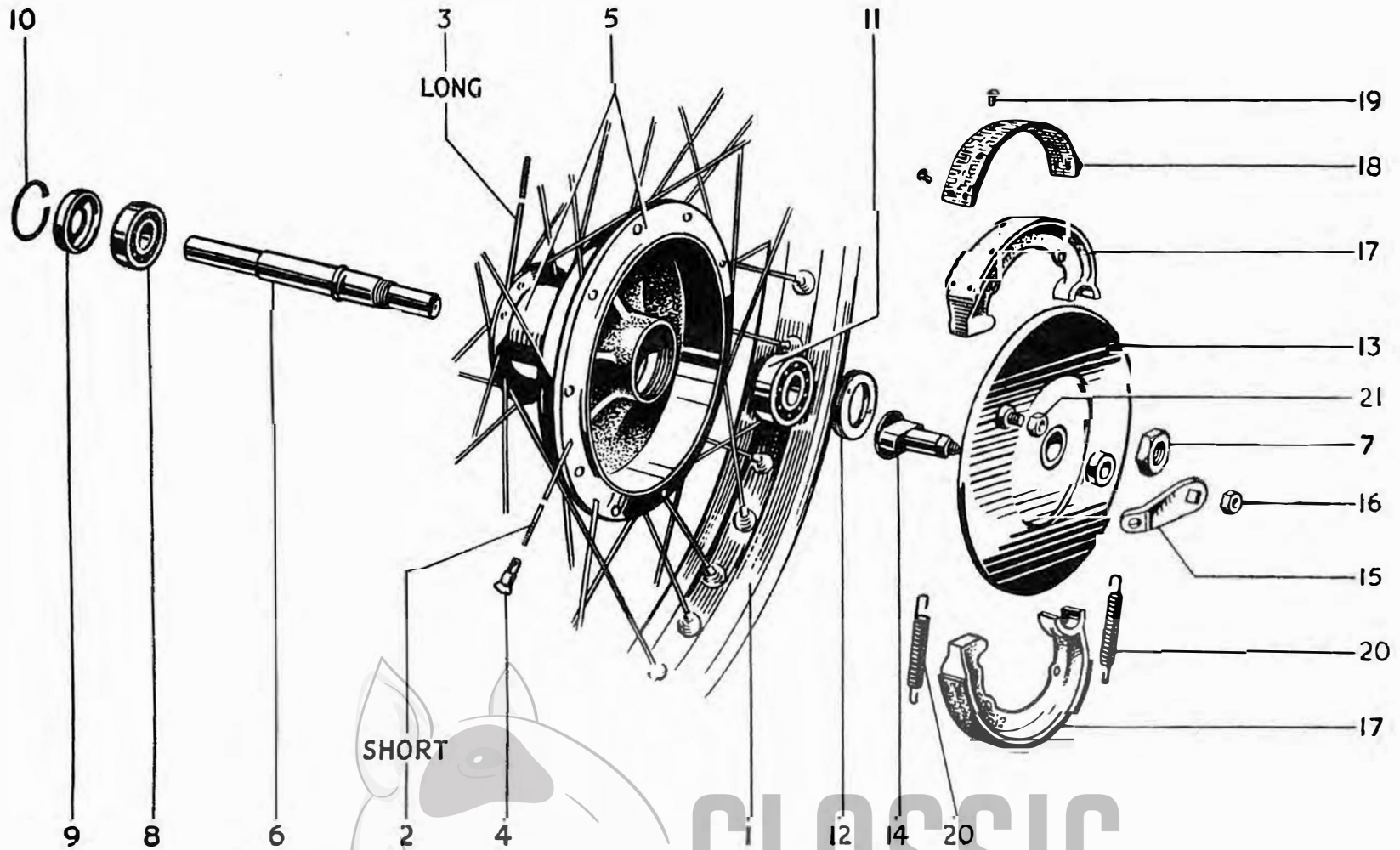
FIG. 7. FRONT WHEEL.
