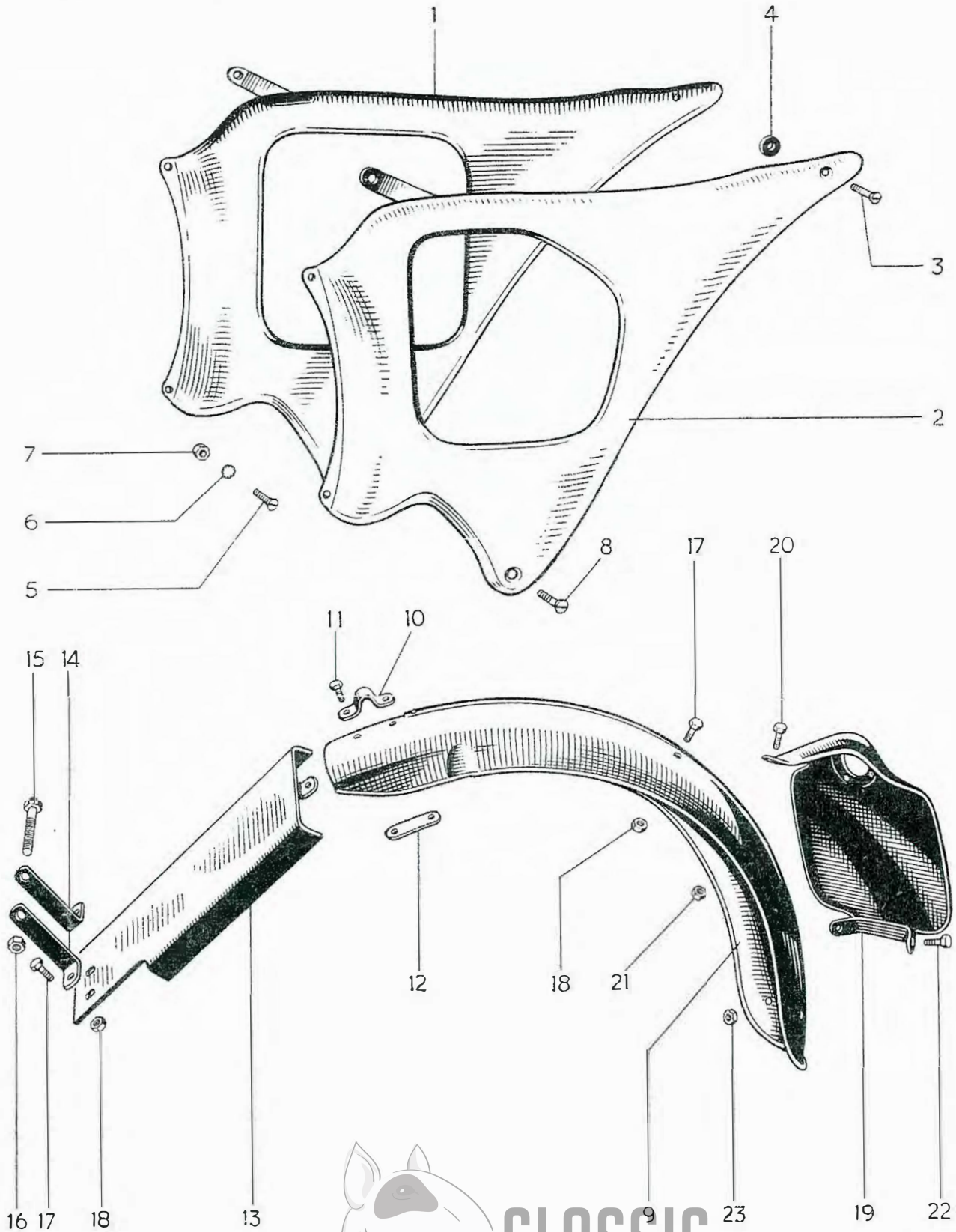
FIG. 10. REAR PANELS.
