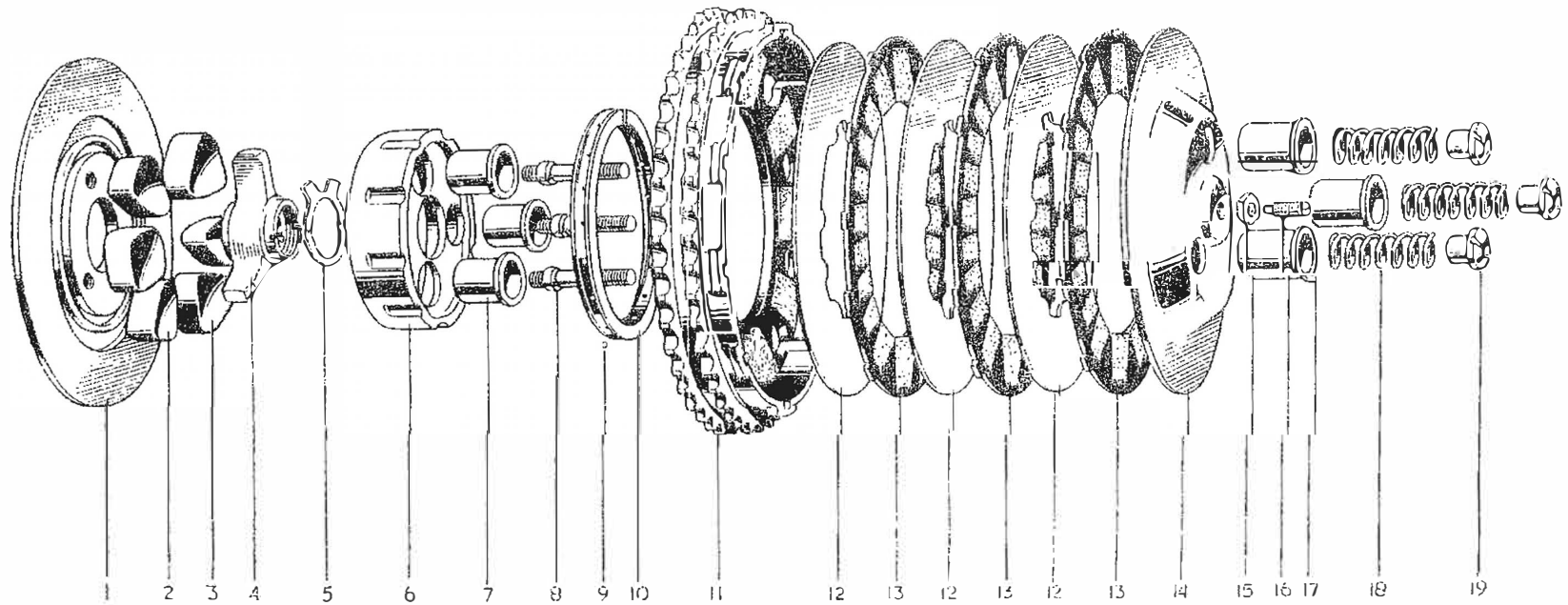
FIG. 3. CLUTCH AND SHOCK ABSORBER UNIT.
