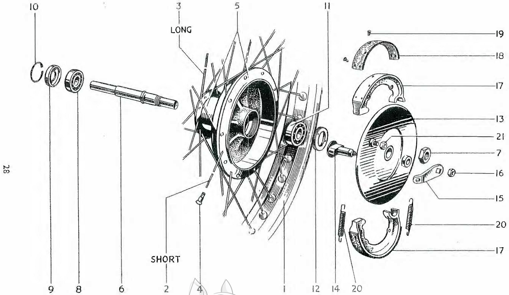
FIG. 7. FRONT WHEEL.
