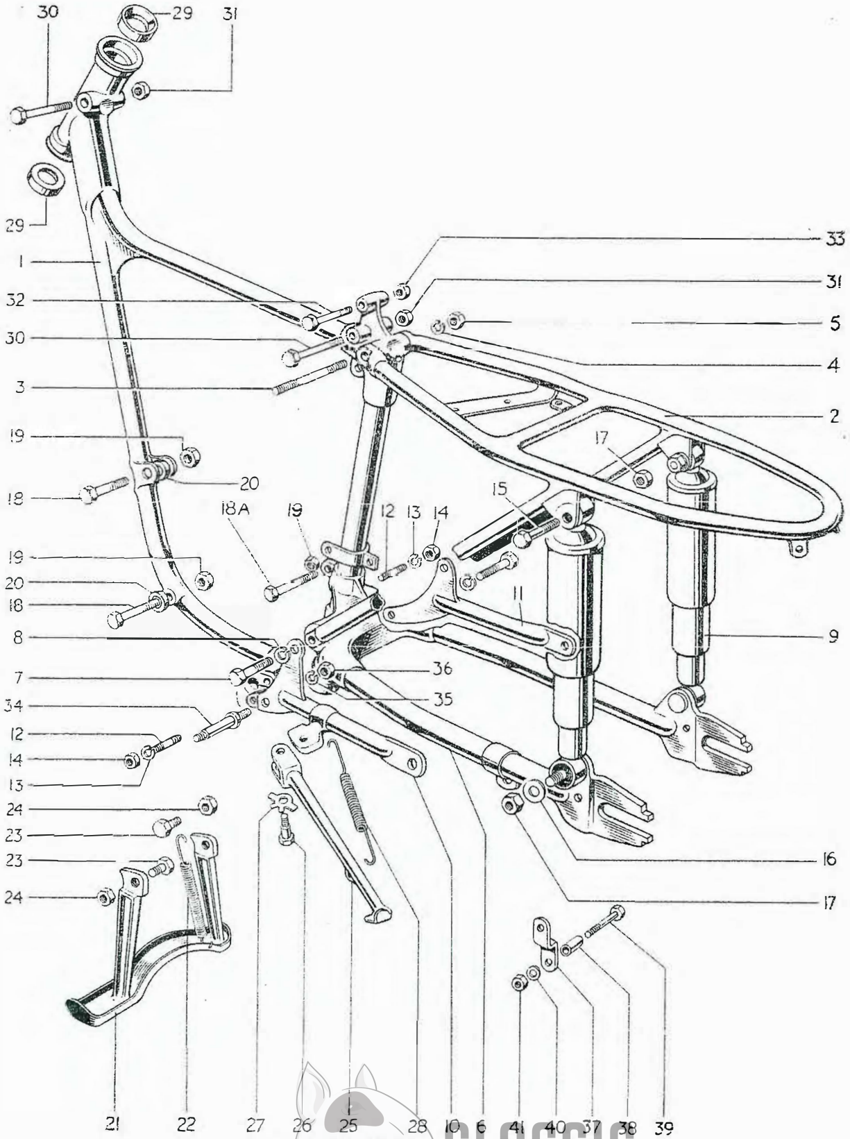
FIG. 4. FRAME AND COMPONENTS. For Index See Page 21.
