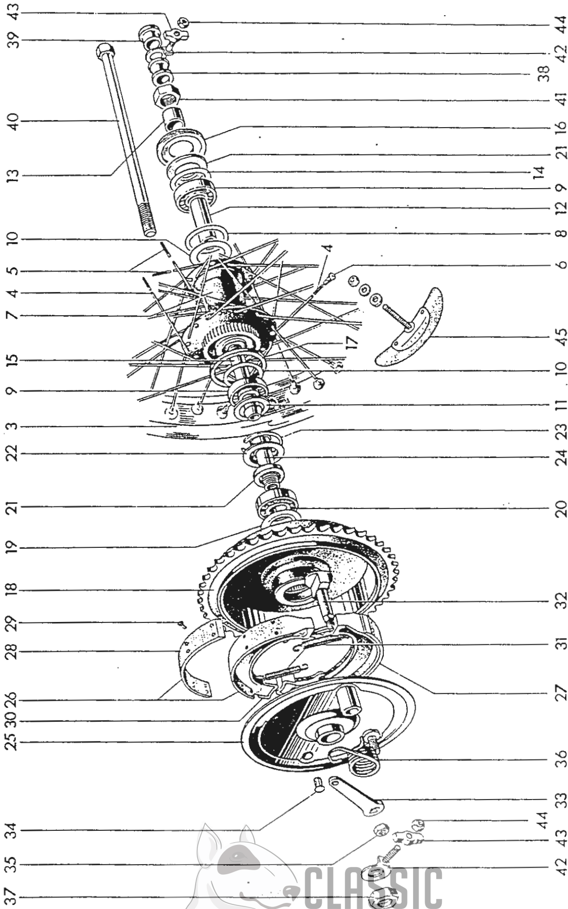
Fig. 21. QUICKLY DETACHABLE REAR WHEEL
