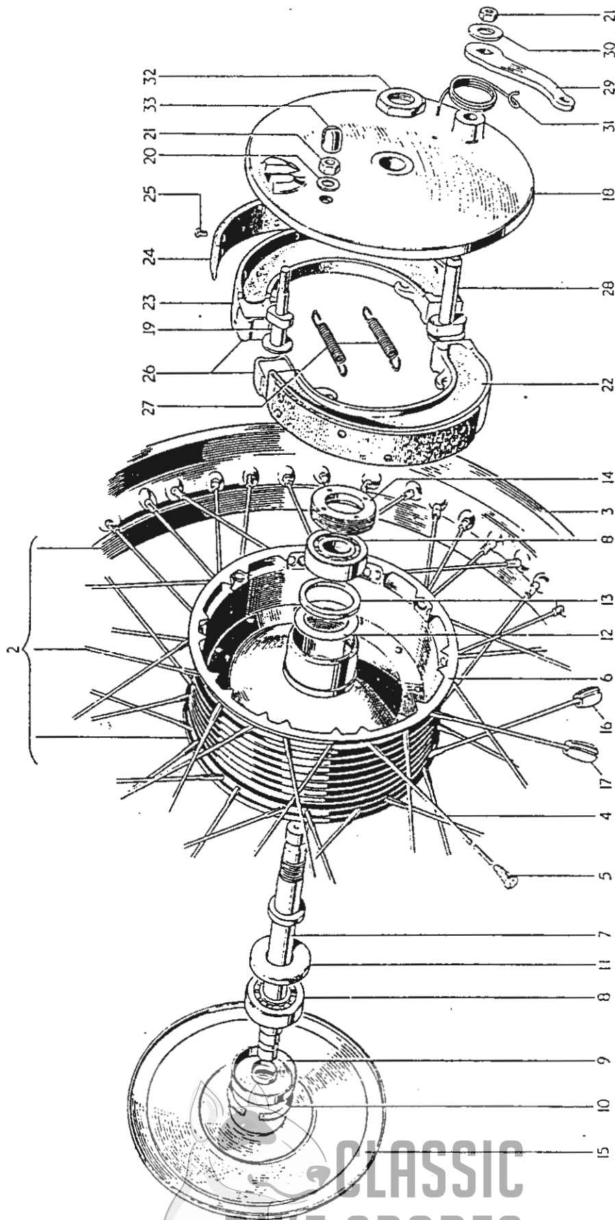
FIG. 19. FRONT WHEEL
