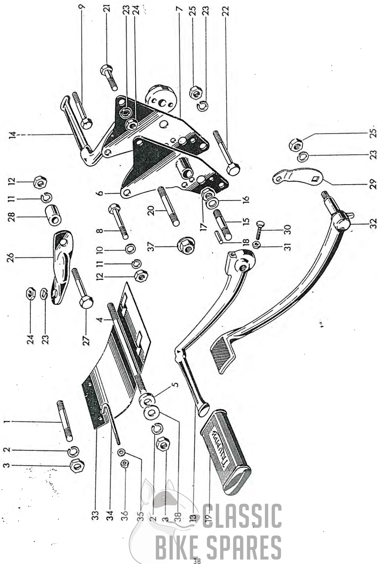
Fig. 14. ENGINE UNIT FITTINGS AND FOOTRESTS
