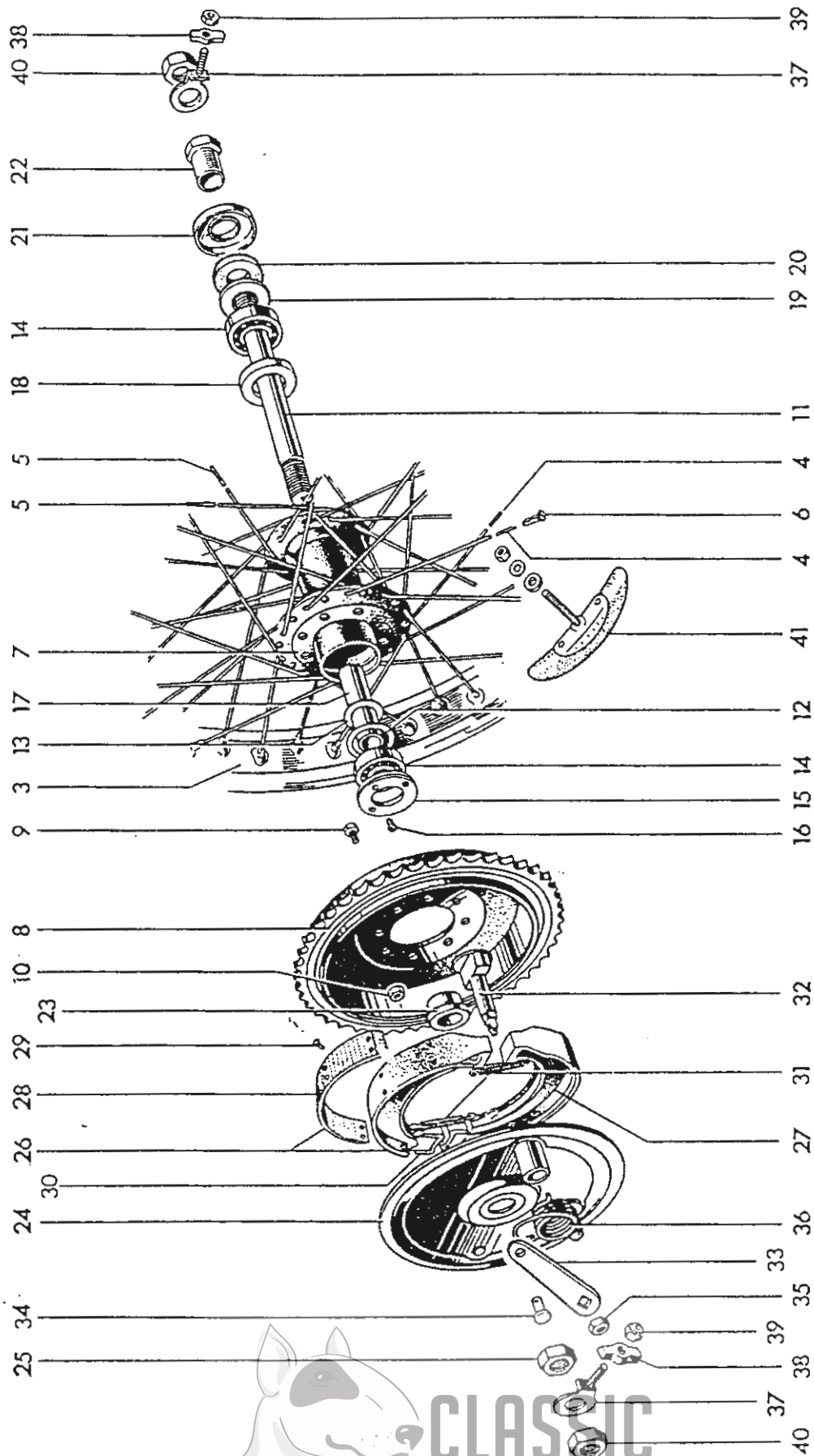
Fig. 20. REAR WHEEL
