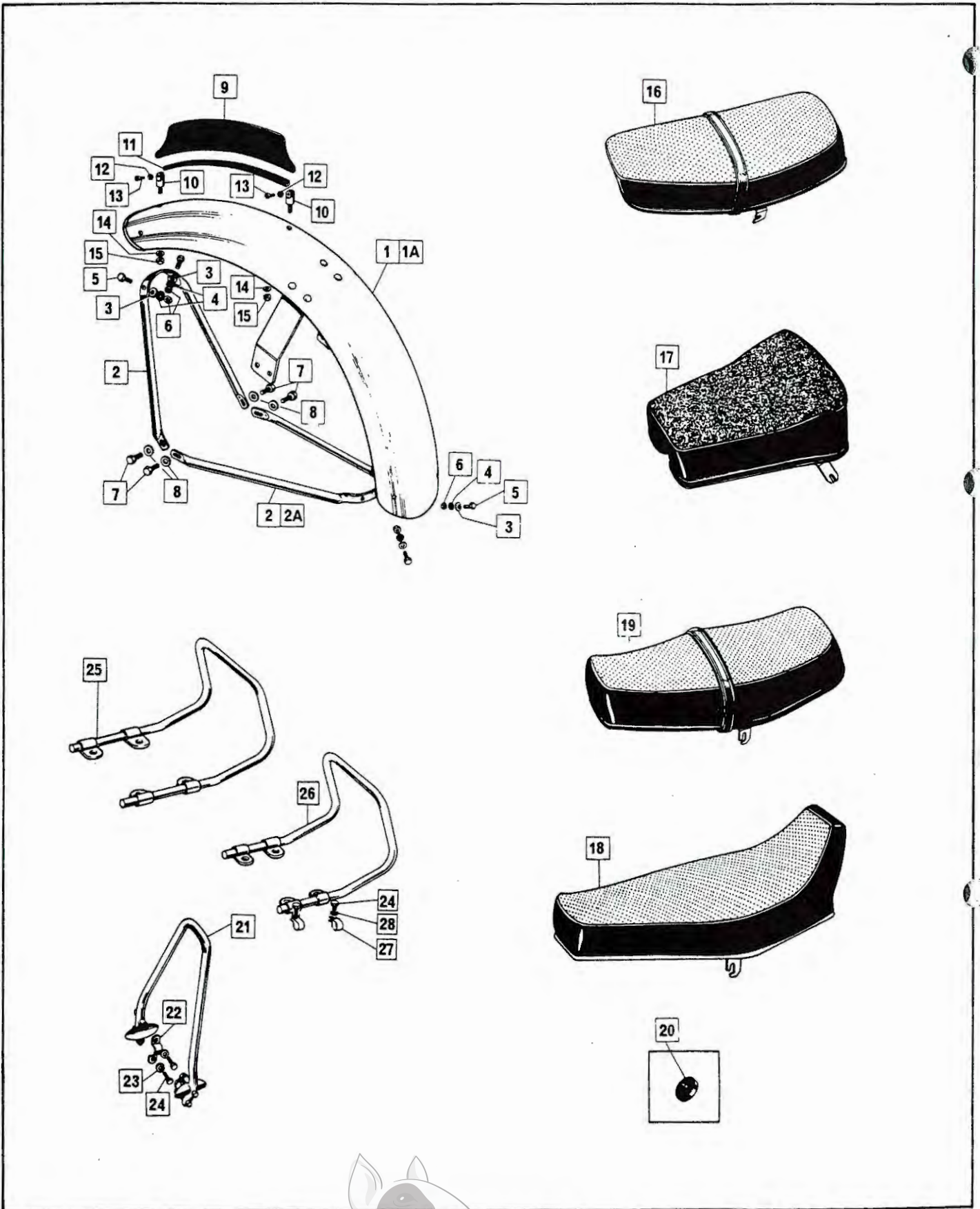
Front Fender, Number Plate and Seats
