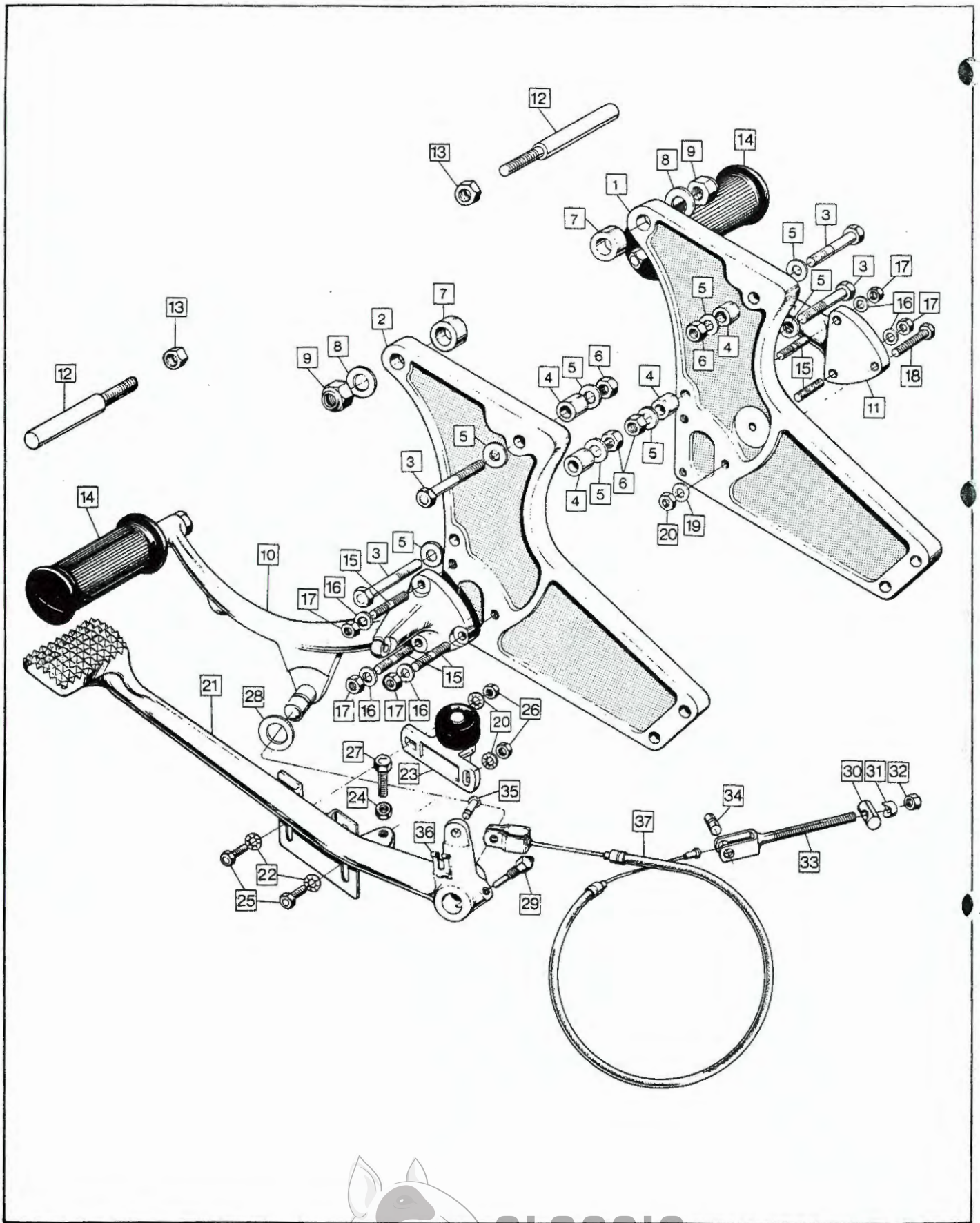
Support Plates, Riders Footpegs, Rear Brake Pedal and Linkage
