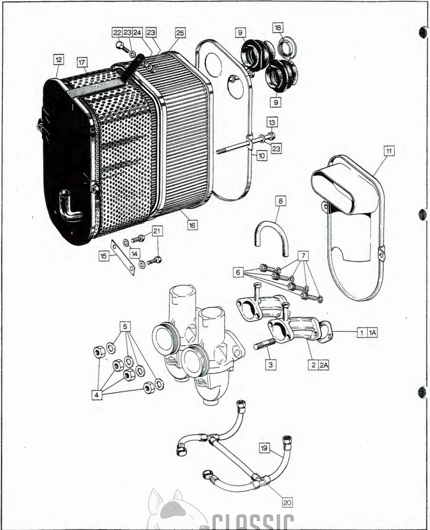
CLASSIC BIKE SPARES Carburetor Mountings, Air Filter and Fuel Line
