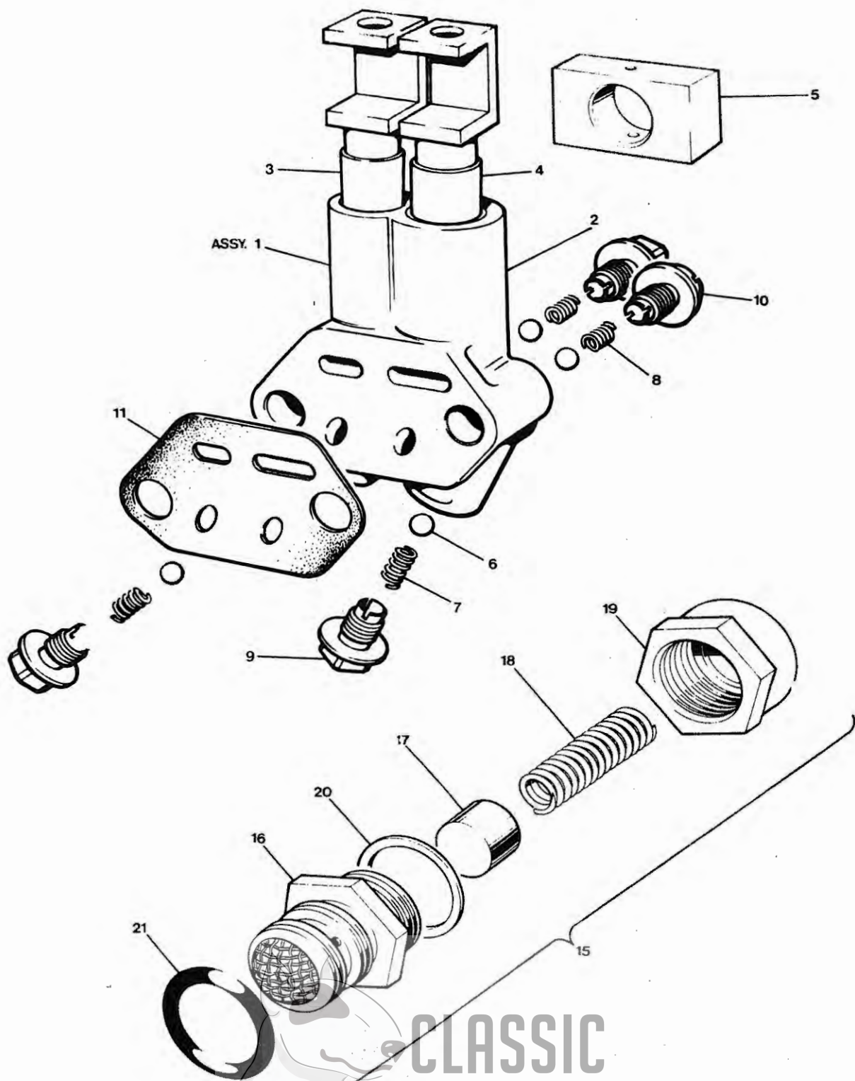
Fig. 3. OIL PUMP AND RELEASE VALVE
