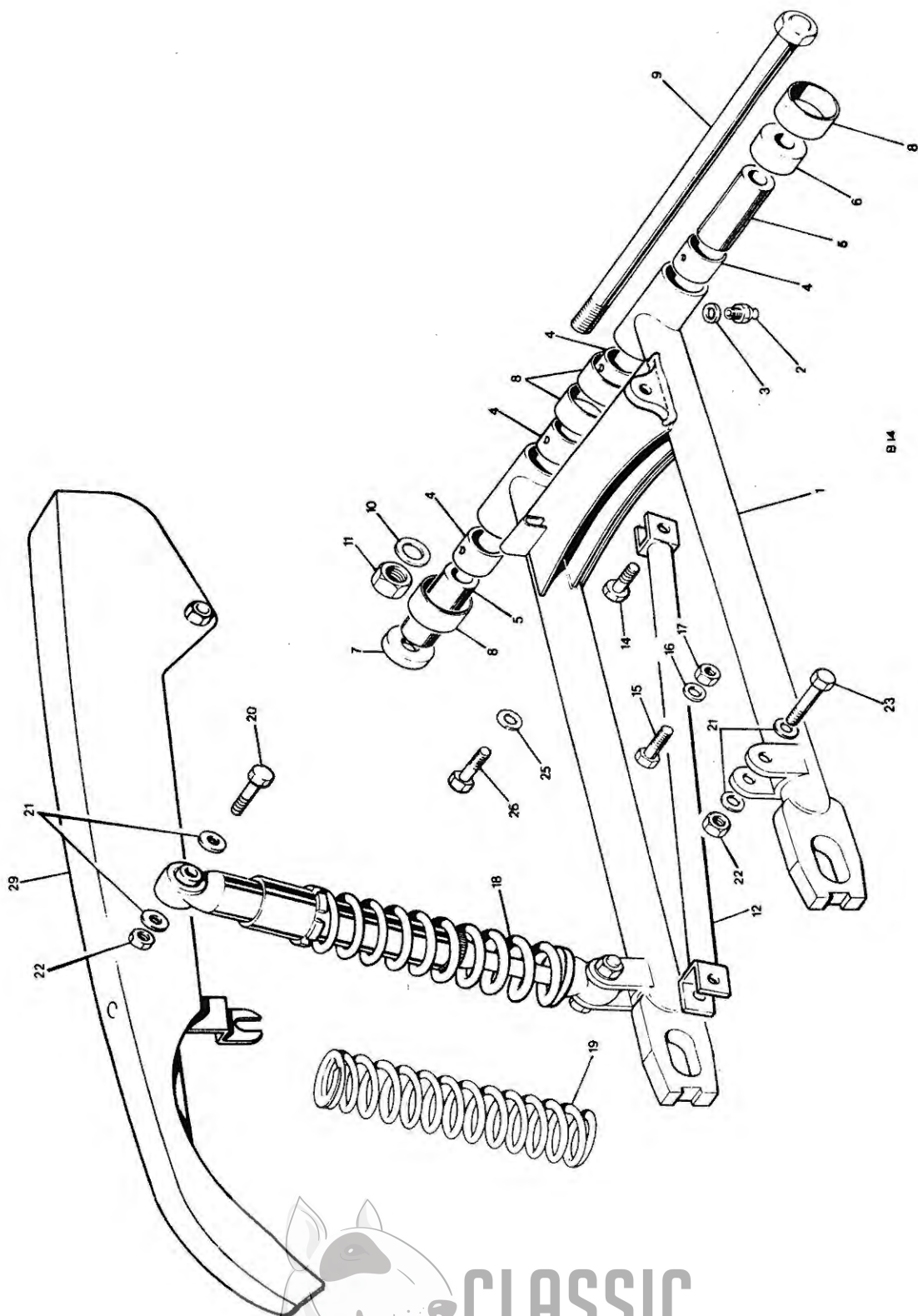
SWINGING ARM AND SUSPENSION UNITS
