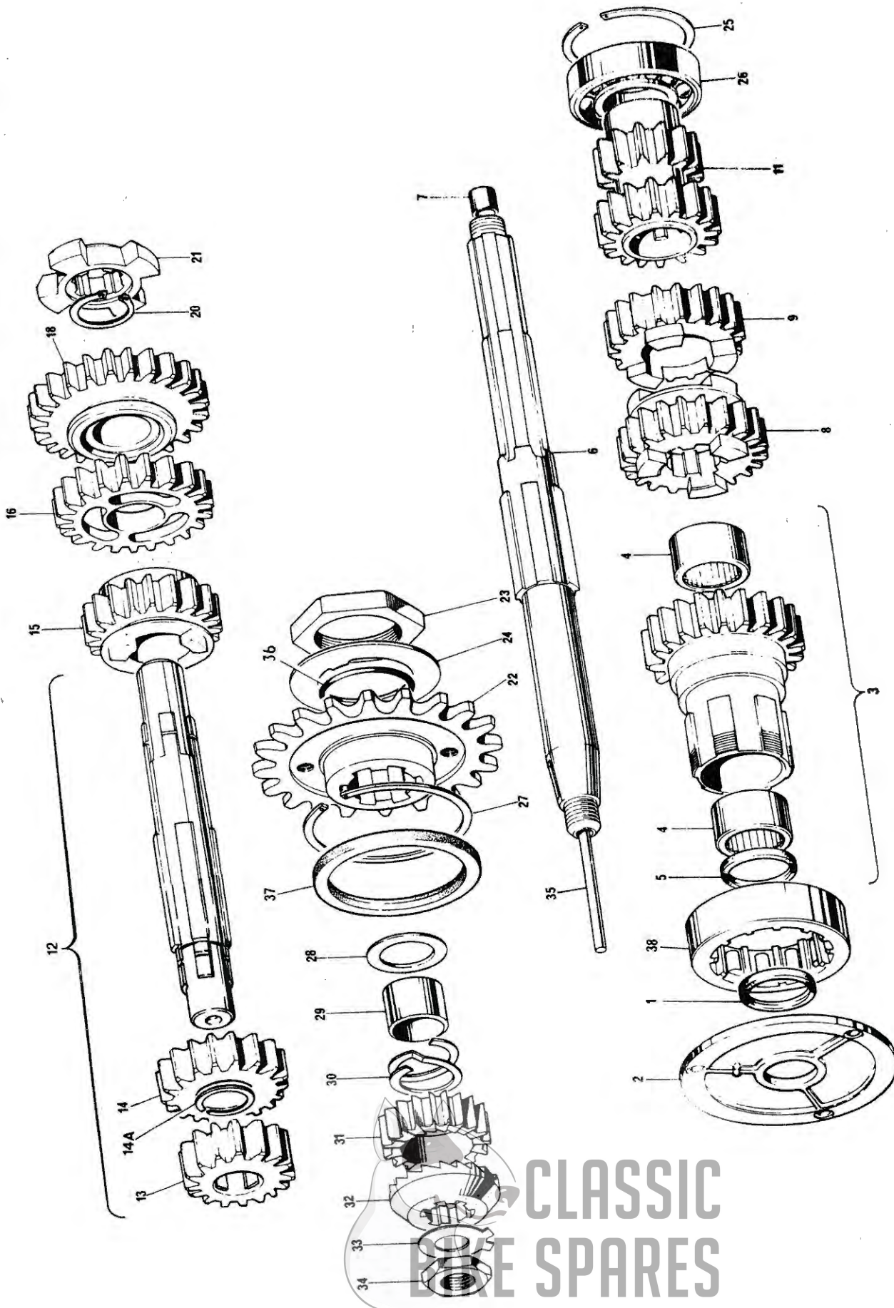
GEARBOX SHAFTS AND GEARS
