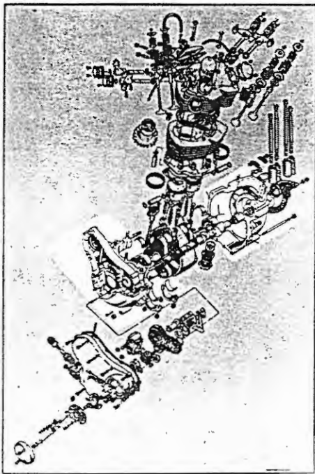
Engine: Crankcases, Crankcase Breather, Tachometer Drive
